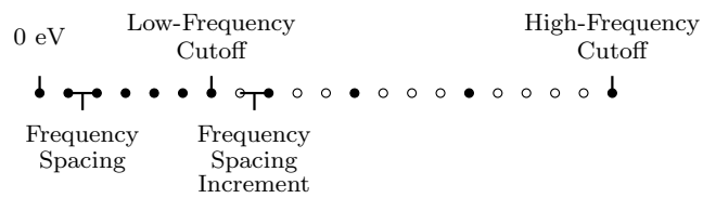
Figure 7: Schematic of the frequency-grid parameters for a full-frequency calculation in epsilon . The open circles are a continuation of the uniform grid that are omitted above the low-frequency cutoff.
