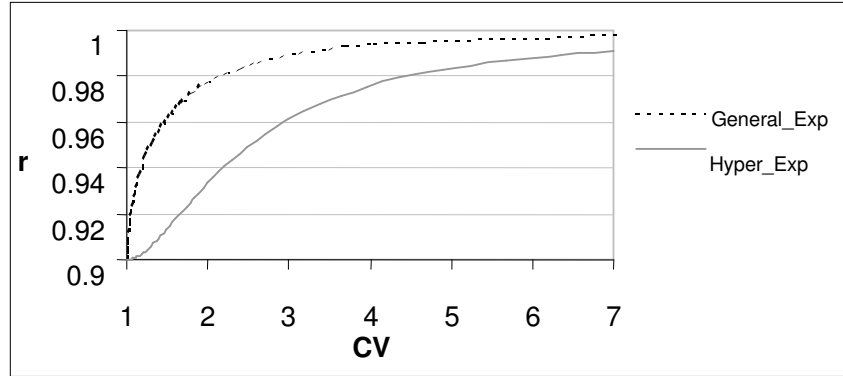
Fig.4 : The r parameters of the GE/M/1 and the H_2/M/1 Make-to-Stock Queues as a function of the inter-arrival time Coefficient of Variation (for \rho=0.9 ).
