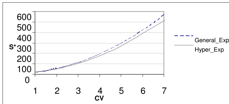
Fig.3 : Comparison Between the Optimal Base Stock Levels of the GE/M/1 and the H_2/M/1 Make-to-Stock Queues ( \rho=0.9 , h=1 , b=10 )
