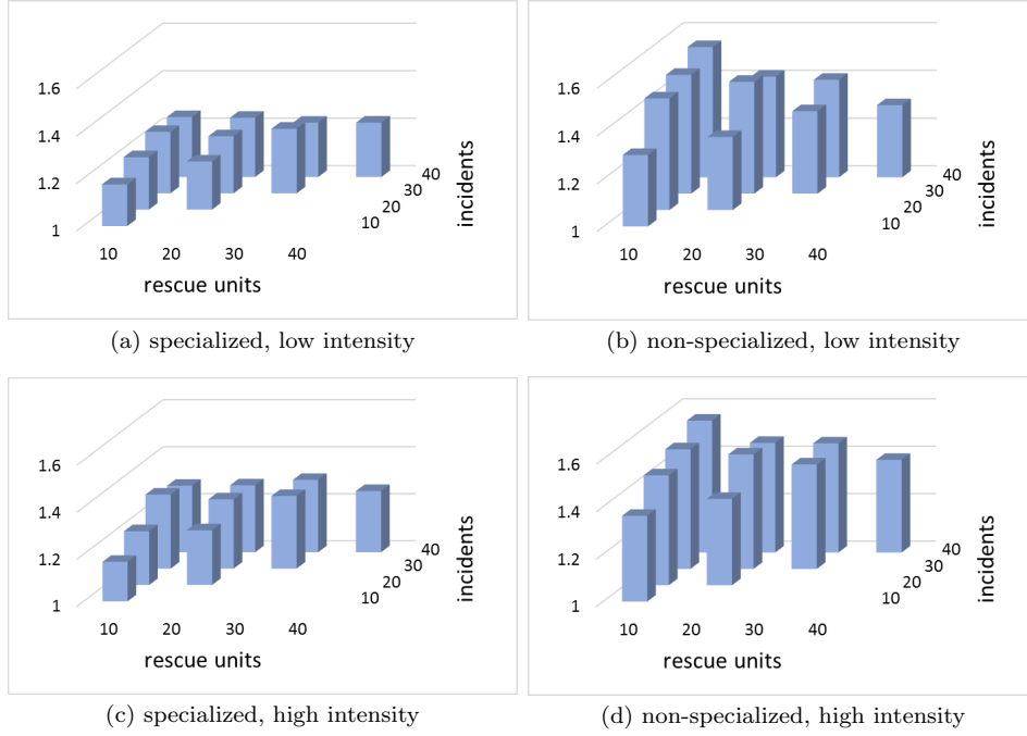
Figure 4: Average ratio of SCHED objective value to optimal objective value
