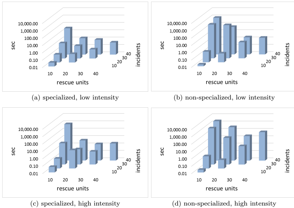
Figure 3: Average execution times of the b&p algorithm
