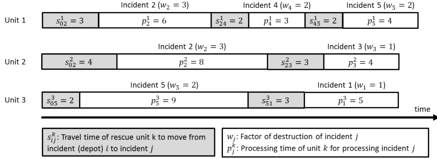
Figure 2: Sample schedule with n = 5 incidents and m = 3 rescue units
