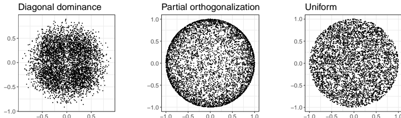
Figure 2: Scatter plot of the two non-zero entries for correlation matrices sampled from \mathcal{E}^3(G) , with G as in Figure 1.
