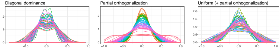
Figure 3: Marginal densities of the non-zero entries of matrices sampled from \mathcal{E}^{50}(G) ; where G is a random graph with 50 vertices and probability of edges 0.05. The first entry in the lower triangle (2, 1) corresponds to the red colour, while the last entry in the last row of the lower triangle (50, 49) corresponds to the pink colour.
