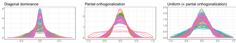
Figure 4: Marginal densities of the non-zero entries of matrices sampled from \mathcal{E}^{50}(G') ; where G' is the chordal graphs obtained as the triangulation of a random graph with 50 vertices and probability of edges 0.05. The first entry in the lower triangle (2, 1) corresponds to the red colour, while the last entry in the last row of the lower triangle (50, 49) corresponds to the pink colour.
