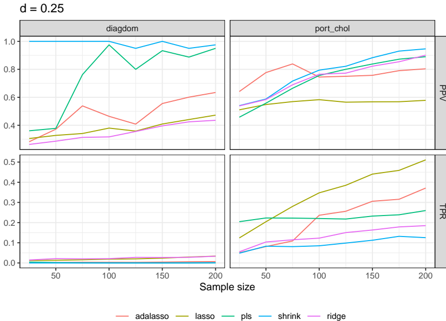
Figure 7: True positive rate (TPR) and true discovery rate (PPV) of the structure learning algorithms for concentration graphs validated in (Kramer et al., 2009), for the highest density, 0.25. The number of variables (vertices in the undirected graph and dimension of the generated matrices) is fixed at 100. adalasso : Adaptive l_1 regularization; lasso : l_1 regularization; pls : partial least squares regression; shrink : shrinkage estimator of Schafer and Strimmer (2005b); ridge : l_2 regularization; diagdom : Diagonal dominance sampling method; port_chol : Uniform sampling with partial orthogonalization of the Cholesky factor.
