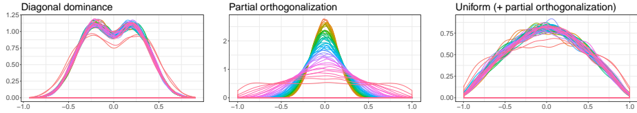
Figure 6: Marginal densities of the non-zero entries of matrices sampled from \mathcal{E}^{50}(G_{chain}) . The first entry in the lower triangle, (2, 1), corresponds to the red colour, while the last entry in the last row of the lower triangle, (49, 48), corresponds to the pink colour.
