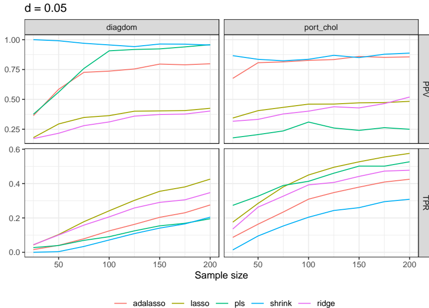
Figure 8: True positive rate (TPR) and true discovery rate (PPV) of the structure learning algorithms for concentration graphs validated in (Krämer et al., 2009), for the lowest density, 0.05. The number of variables (vertices in the undirected graph and dimension of the generated matrices) is fixed at 100. adalasso : Adaptive l_1 regularization; lasso : l_1 regularization; pls : partial least squares regression; shrink : shrinkage estimator of Schäfer and Strimmer (2005b); ridge : l_2 regularization; diagdom : Diagonal dominance sampling method; port_chol : Uniform sampling with partial orthogonalization of the Cholesky factor.
