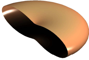
Figure 1: In this table, we report the condition number of the operator \mathcal{L} , which we have computed numerically as a function of the spatial discretization points for the vesicle geometry depicted to the left.
