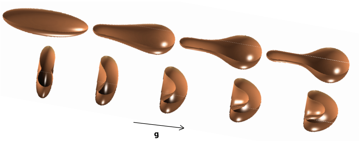
Figure 8: Snapshots of a deforming prolate and an oblate vesicle suspended in a viscous fluid in the presence of gravity. In this example, the reduced volumes of the prolate of the oblate vesicles are 0.78 and 0.65 respectively; \hat{g} = 100 .
