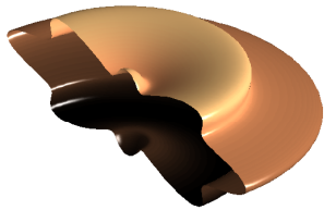
Figure 3: Relative errors in computing the curvatures numerically on the shape shown. The reference values are computed analytically. As expected, we observe spectral convergence.
