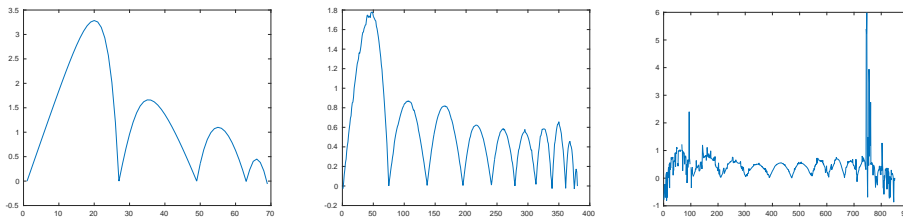
FIGURE 1. Difference \min \mathbf{Q}_+ - \min \text{LP} with n=(4,10,15) ; One reads b + |\mathbf{a}| on the x -axis
