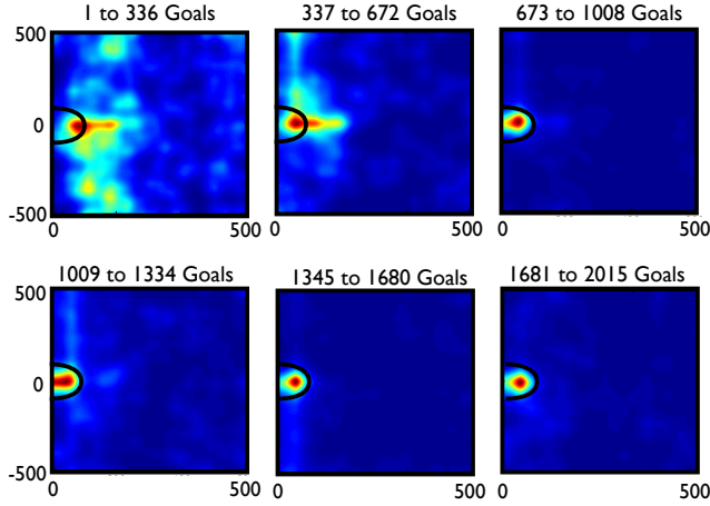
Figure 9: Histograms of self-generated goals displayed over time windows indexed by the number of performed goals, for an experiment of 30000 microactions on a 15 DOF arm, for a high-volume task space S = [-500; 500] \times [0; 500] , according to the reachable space contained in [-50; 50] \times [0; 50] (the black half-circle represents the contour of the area reachable by the arm according to its length of 50 units).
