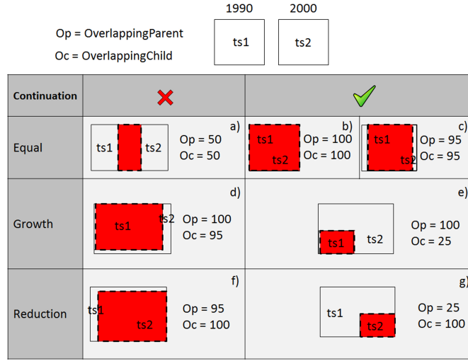
Figure 9: The detection and qualification of continuation relationships
