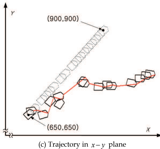
Fig. 7. The dead-reckoning navigation.
