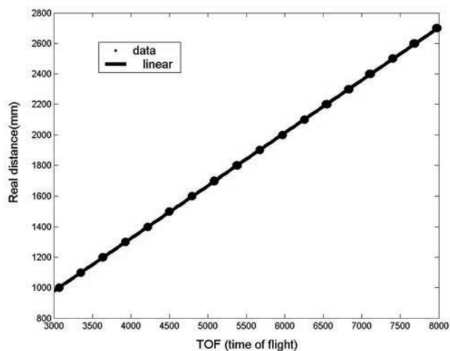
Fig. 5. Real distance with respect to ultrasonic TOF.
