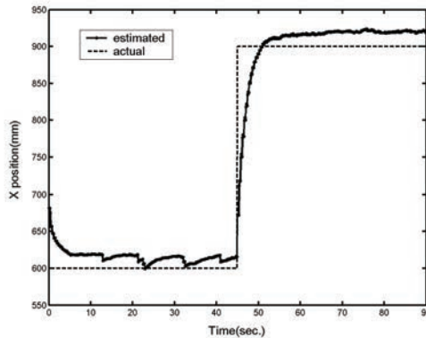
(a) Position estimation in x axis.
