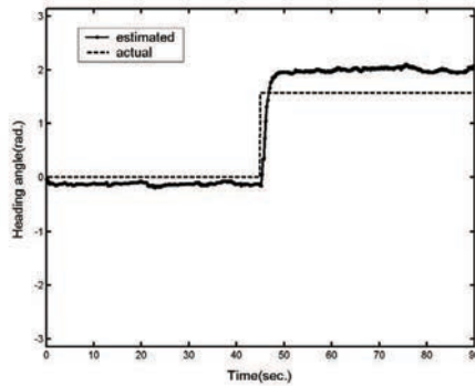
(c) Estimation for heading angle.
