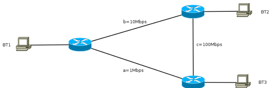
Figure 2: Example topology
