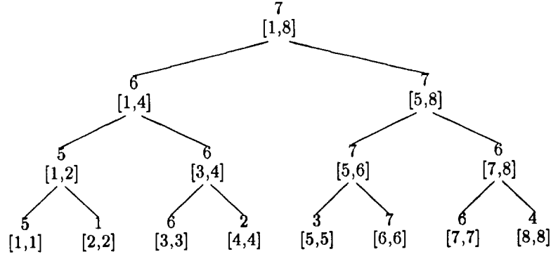
Figure 5: Search tree identifying maximum values over subintervals, which is used to solve the nearest right neighbor problem.
