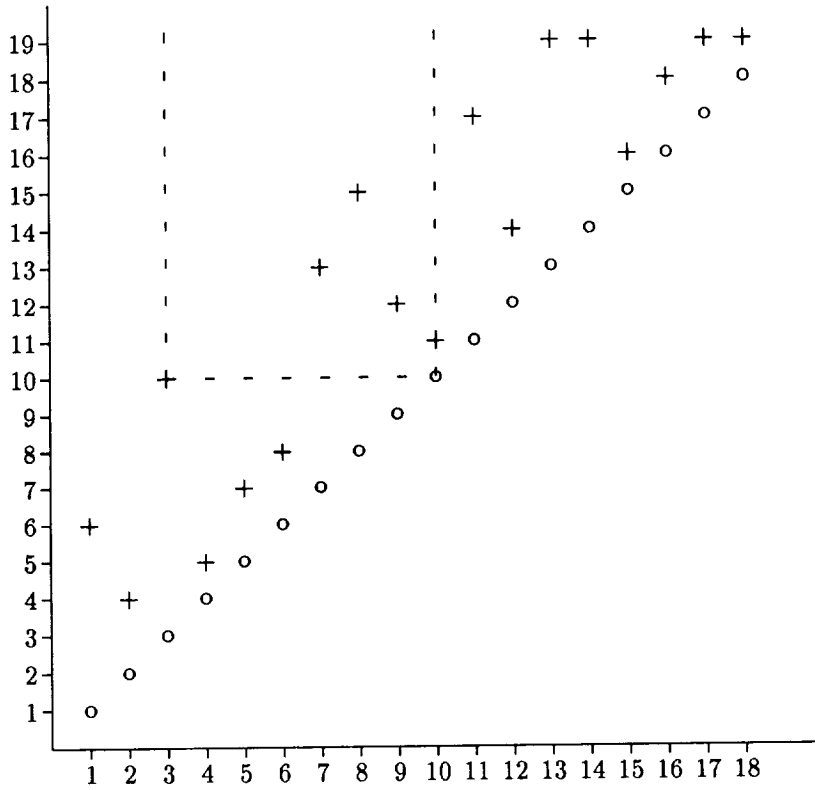
Figure 2: The trace of Figure 1 is repeated, along with corresponding next and prev values. The values (t, next(t)) are plotted as +’s, and the values (t, t) as o’s. The number of points strictly within the rectangle indicated by dashed lines is one less than the stack distance of x_{10} = b .
