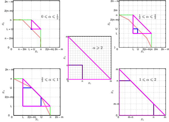
Fig. 1. Illustration of \mathcal{C} (red dotted line), \mathcal{C}_{NE} (solid blue line), \mathcal{C}_{FB} (green dotted line), and \mathcal{C}_{FB/NE} (magenta solid line) in all interference regimes.
