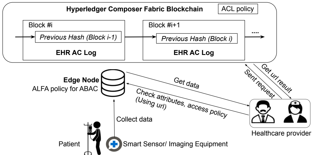
Fig. 4: Hybrid architecture of blockchain and edge node.
