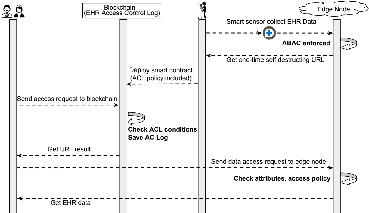
Fig. 5: Access control workflow.
