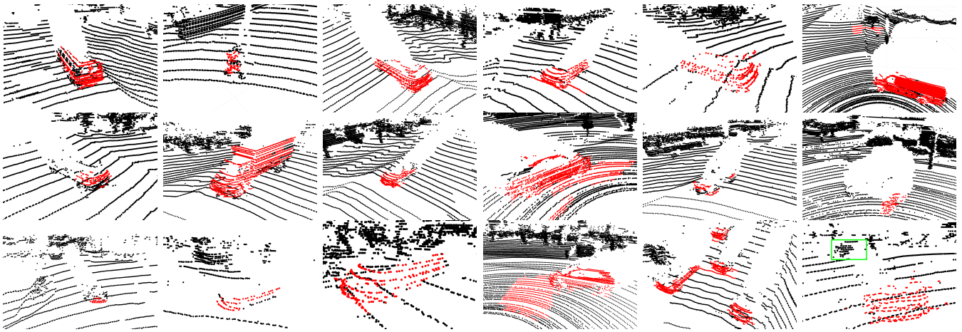
Fig. 8: Real data examples (22 dynamic objects) of our detection method. False detections can occur (row 1, col. 6), but rarely persist in the next scan. Inaccurate surface normals cause incomplete region growth (col. 1 and 2) or growth to static points (col. 4). The green box in the last image indicates an unlabelled dynamic object due to occlusion by the other object in the freespace scan(s). The example in row 2, col. 6 is a barely visible vehicle due to many faulty returns.
