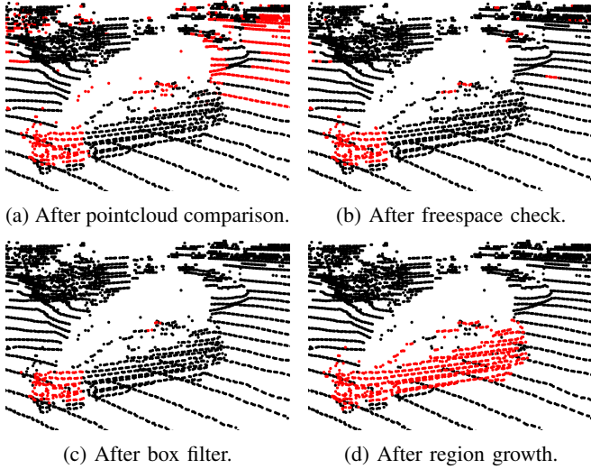
Fig. 3: A vehicle throughout the detection pipeline. Refer to the pipeline in Fig. 2 for corresponding letters (a) to (d).
