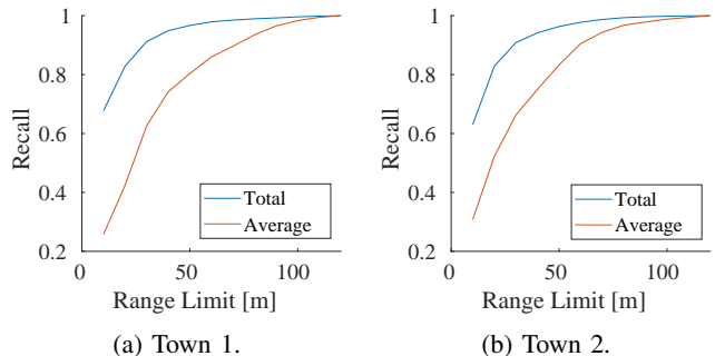
Fig. 7: Recall ( total and average - see Eq. 3 and 4) using groundtruth labels on two simulated sequences with varying limited range. Total recall is high at low range limits because nearby objects have more points, downplaying far-away ones.
