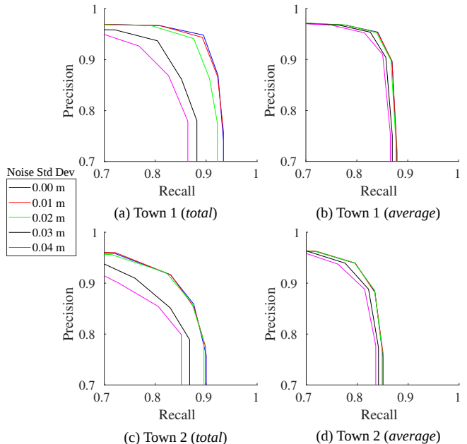
Fig. 6: Precision-recall plots ( total and average - see Eq. 3 and 4) on two simulated sequences. The standard deviation of range measurement noise was varied. Note that a Velodyne HDL-64E has a standard deviation rated less than 0.02 m.
