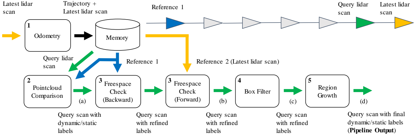
Fig. 2: The pipeline describes the sequence of operations on the lidar scan of interest ( query scan ), outputting the scan with points labelled dynamic or static. A lidar odometry algorithm computes the sensor trajectory, which aligns the latest scan . The labels (a) to (d) correspond to the images in Fig. 3. The numbers correspond to the enumerated steps in the text.
