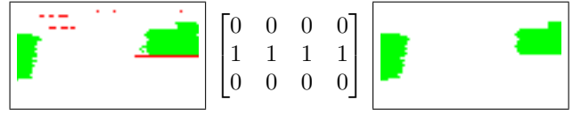
Fig. 5: We apply a filter (middle) to a scan’s image representation to remove mislabelled dynamic points (red) while maintaining correct ones (green). We show a before (left) and after (right) example (64 lasers, limited horizontal FOV).
