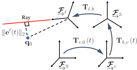
Fig. 4: A visualization of the point-to-line distance (see Eq. 1). \mathbf{T}_{v,0} is the sensor trajectory, \mathbf{T}_{h,v} is the spinning lidar rotation, and \mathbf{T}_{\ell,h} is the unique pose for laser \ell . We require the time, t , and laser, \ell , combination that minimizes \|\mathbf{e}^\ell(t)\|_2 .
