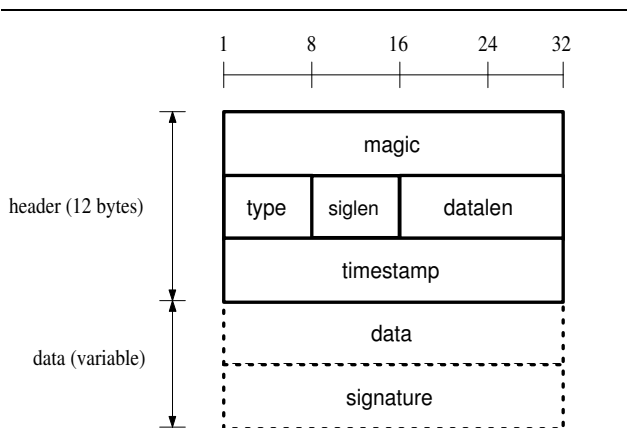
Figure 1. S-ARP packet extension.
