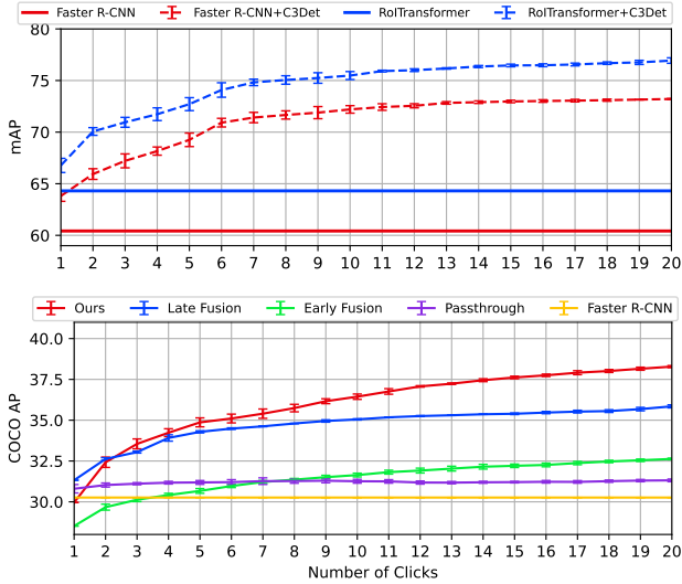
Figure 14. Performance on Tiny-DOTA. Top: Both Faster R-CNN and RoI Transformer [10] (solid lines) are improved by adding C3Det (dashed lines). Bottom: Our method against Faster R-CNN baselines measured with COCO AP@[.50:.05:.95].
