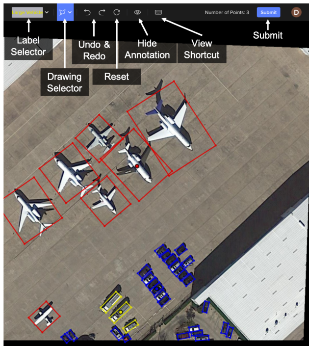
Figure 12. User Study Frontend. Our user-study GUI in semi-automatic annotation mode. Annotator inputs are shown as dots, while model predicted bounding boxes are drawn as quadrilaterals.
