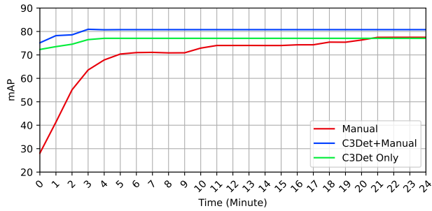
(a) IoU threshold for mAP = 0.1
