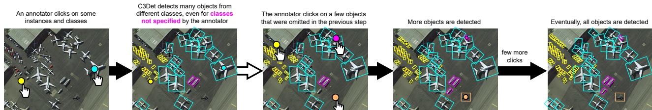
Figure 1. C3Det is a deep learning framework for interactive tiny-object detection that relates multiple annotator clicks to multiple instances and multiple classes of objects (each object class is depicted with a different color), in order to reduce overall annotation cost.
