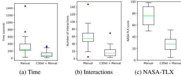
Figure 9. Box plots of per-sample (a) time taken and (b) number of interactions, and overall (c) task load assessed using NASA-TLX.
