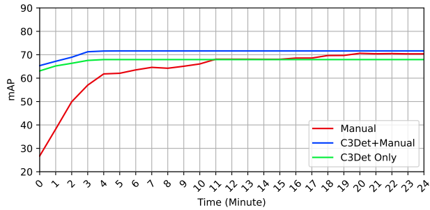
(b) IoU threshold for mAP = 0.5
