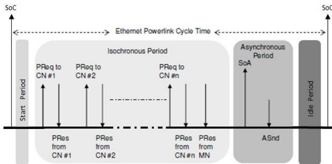
Fig. 2. Ethernet Powerlink cycle.
