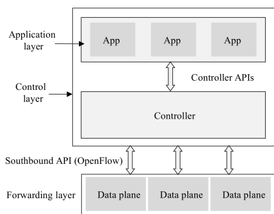
Fig. 1. SDN architecture
