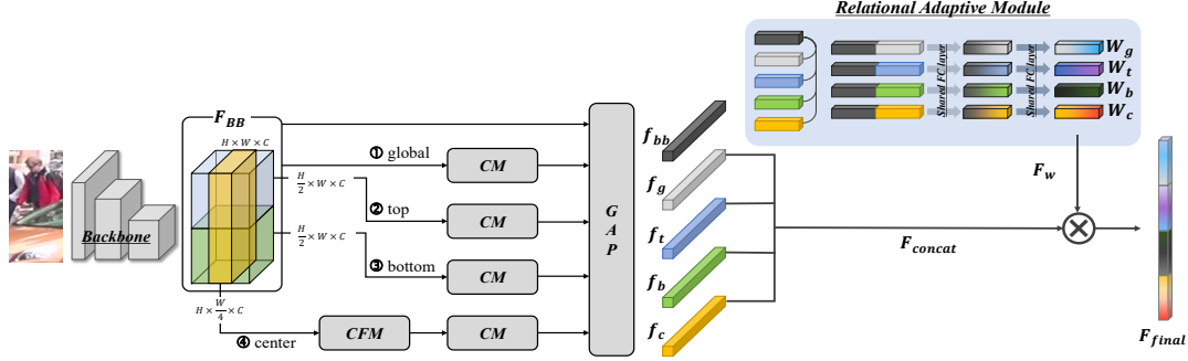
Fig. 2: Overall framework of the proposed approach. OCNet consists of Converter Module (CM), Center-Focus module (CFM), and Relation Adaptive Module (RAM). The backbone feature F_{BB} go through CM to extract global features f_g , top features f_t , bottom features f_b , and center features f_c . After passing through RAM, it becomes a relational-weight F_w with the same size as F_{concat} . Multiplying these two results in a final representation feature that is well-aligned and robust to occlusion.
