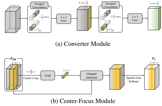
Fig. 3: Overview of our (a) Converter Module (CM) (b) Center-Focus Module (CFM).
