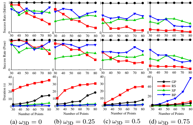
(a) \omega_{3D} = 0 (b) \omega_{3D} = 0.25 (c) \omega_{3D} = 0.5 (d) \omega_{3D} = 0.75 Figure 7. Mean success rates and median runtimes with respect to the number of random 3D points and the 3D outlier fraction, for 50 Monte Carlo simulations per parameter value with the torus prior.
