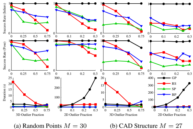
(a) Random Points M = 30 (b) CAD Structure M = 27 Figure 8. Mean success rates and median runtimes with respect to the 3D and 2D outlier fractions for the random points and CAD structure datasets, for 50 Monte Carlo simulations per parameter value with the torus prior.
