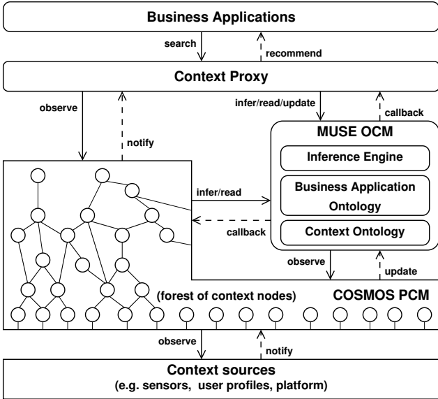
Figure 1. Hybrid architecture
