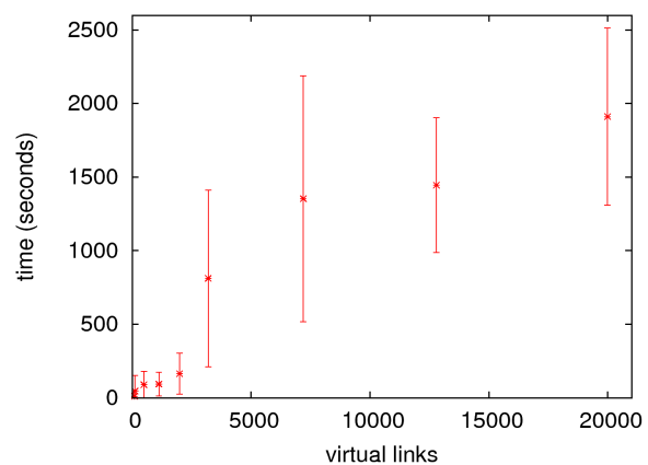
Figure 1. HMN execution time in function of number of virtual links being mapped (torus cluster).
