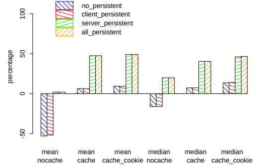
Fig. 9. Latency improvement results for the AT&T Labs–Research trace relative to the no-proxy case.
