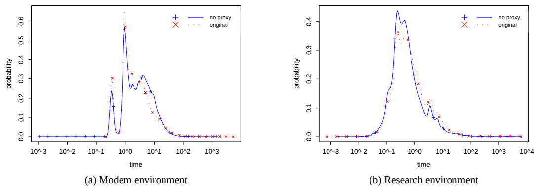
Fig. 4. Simulation validation: total latency.
