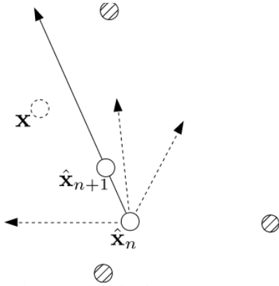
Fig. 6. Illustration of one step of the local optimization process
