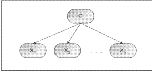
Figure 1. Naive Bayes structure
