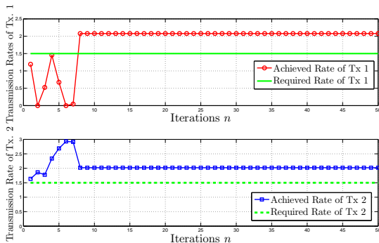
Fig. 5. Instantaneous achieved rates of transmitter 1 (red) and 2 (blue). Here, \text{SNR} = \frac{p_{k, \max}}{\sigma_k^2} = 10 dBs, (\Gamma_1, \Gamma_2) = (1.5, 1.5) bps and N_1 = N_2 = 32 power levels.
