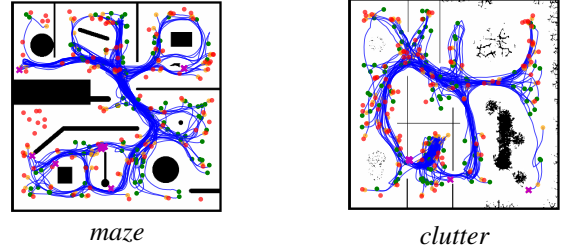
Fig. 5: Evaluation runs between 100 randomly sampled start and target positions on the two unknown test maps (both 10\text{ m} \times 10\text{ m} ). The model used for visualization is c_{1000}+CPO . The trajectories are shown in blue, the starting positions in green, the set targets in red, the trajectory end points in yellow and crashes as magenta crosses.
