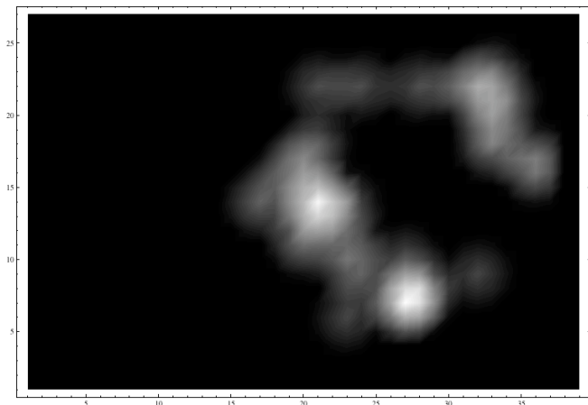
Fig. 19. Two dye track (“blob”) hypotheses computed from the clusters identified in the PDM.
