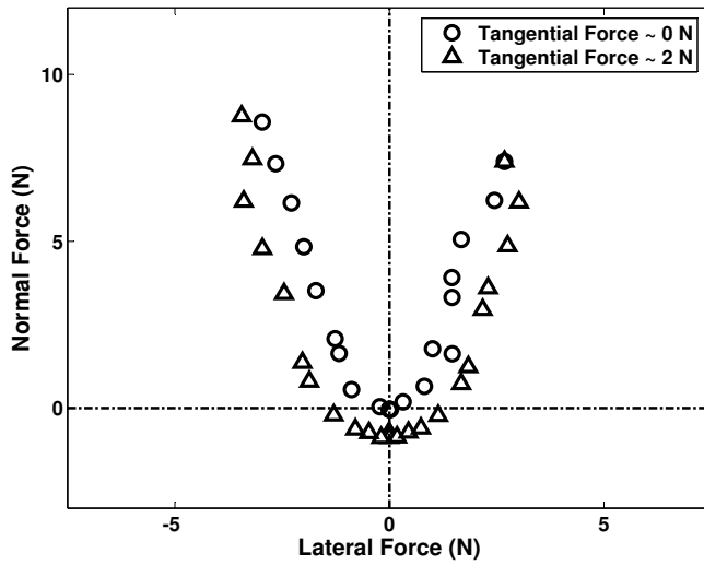
Fig. 5. Contact failure forces for the DPS plotted in the lateral-normal plane are symmetric and similar to previous isotropic adhesion models. When adhesion is initially present due to positive tangential forces, as shown in the lower curve, increasing the lateral force results in decreased adhesion.
