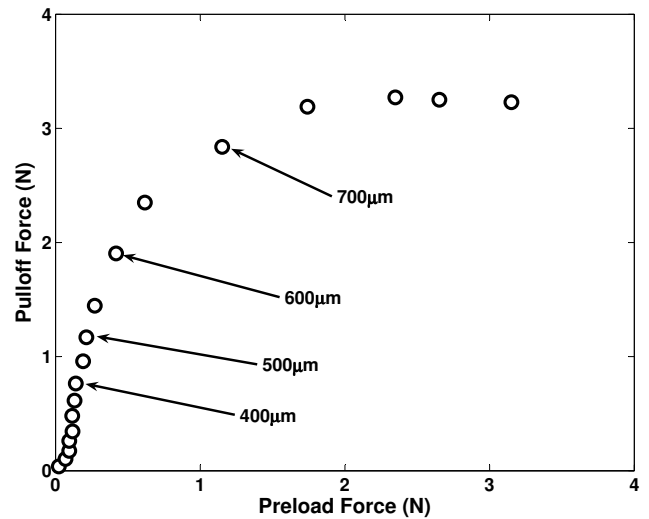
Fig. 3. Pull-off force in the normal direction as a function of preload. The pull-off force begins to saturate at preload forces above \sim 1\text{N} , corresponding to preload depths larger than 700\mu\text{m} .
