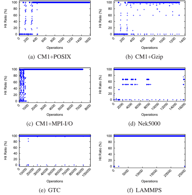
Fig. 5: Measurement of the hit ratio using Omnisc’IO to predict the location of the next accessed segment, as a function of the number of the number of operations completed.
