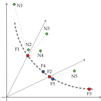
Fig. 3. Demonstration for cascade clustering: Step 1. Frontier identification. The identification divides the population into frontiers (F1 to F5) and nonfrontiers (N1 to N5); Step 2. Cluster and sort the frontiers, locate the cluster centers (F1, F2 and F3). The frontier individuals attached to a mutual reference vector are clustered and sorted using PDM; Step 3. Cluster and sort the nonfrontiers. The nonfrontiers are attached to the clusters and sorted using their distances to the cluster centers; Step 4. Round-robin picking. The next population (F1, F2, F3, N2, N5) is selected by popping the selection queues.
