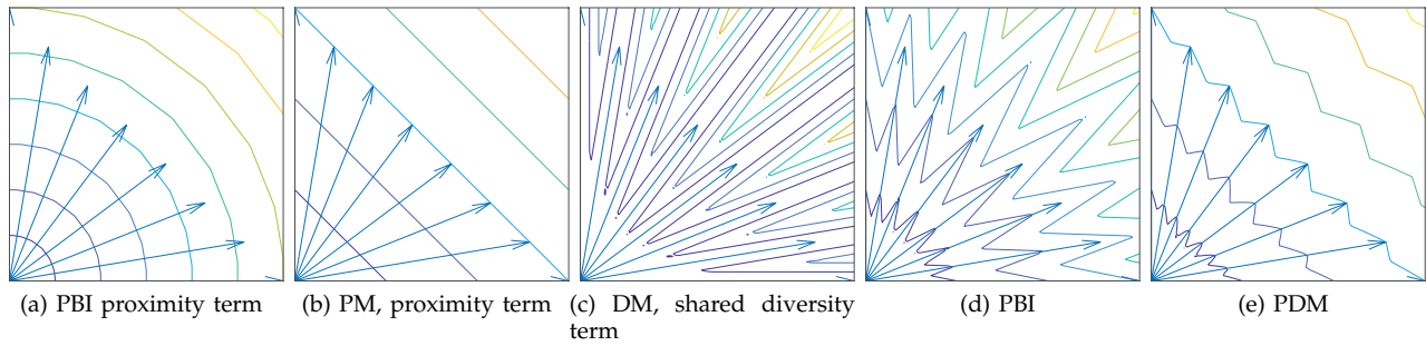
Fig. 2. Fields of PBI function and PDM function in the objective space. We exclude other factors and thus the evolution pressure can be treated as gradients. In (a) and (b), the contours for the proximity term of PBI and PDM is respectively drawn; In (c), the contours for the shared diversity term are, respectively, drawn. In (d) and (e), the contours of the combined PBI field and PDM field are, respectively, illustrated. The contours with the same PBI values fluctuate around concave concentric arcs, while the contours of PDM fluctuate around the parallel lines. PDM has no preference for the PF curvature.
