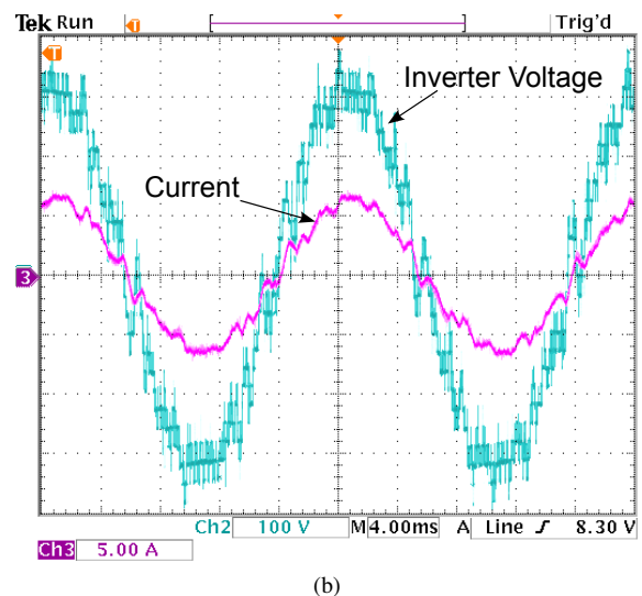
Fig. 14. Current limiting mode applied to grid connection (a) Stable operation ( K_P = 4 ), (b) Unstable operation with higher proportional gain ( K_P = 5 ).
