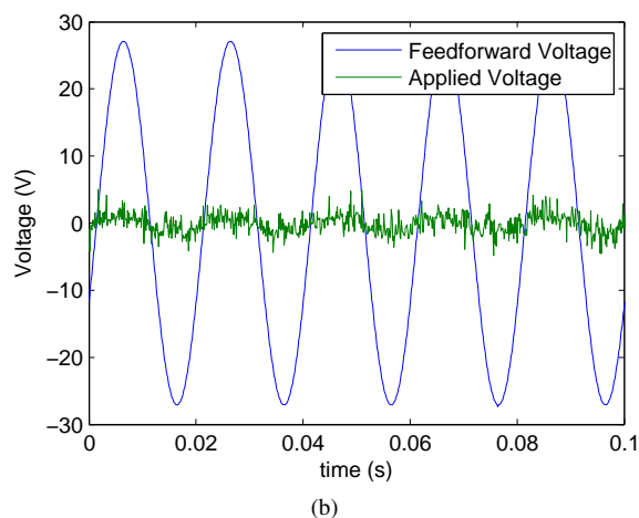
Fig. 13. Behaviour of the current limiting controller with the inverter terminals shorted (a) Measured inverter current and voltage, (b) Feedforward voltage and applied voltage signals per module.
