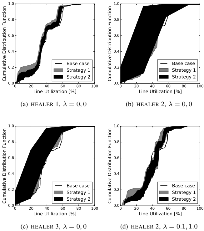
Fig. 7. Lines utilization in case-30 with AC power flow under different healing modes and \lambda values for STRATEGY 1 and STRATEGY 2 respectively.
