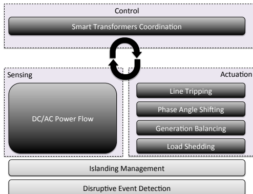
Fig. 1. A model for self-repairable Smart Grids using coordinating smart transformers.
