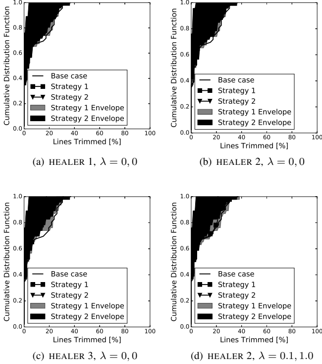
Fig. 4. Lines trimmed in case-39 with AC power flow under different healing modes and \lambda values for STRATEGY 1 and STRATEGY 2 respectively.
