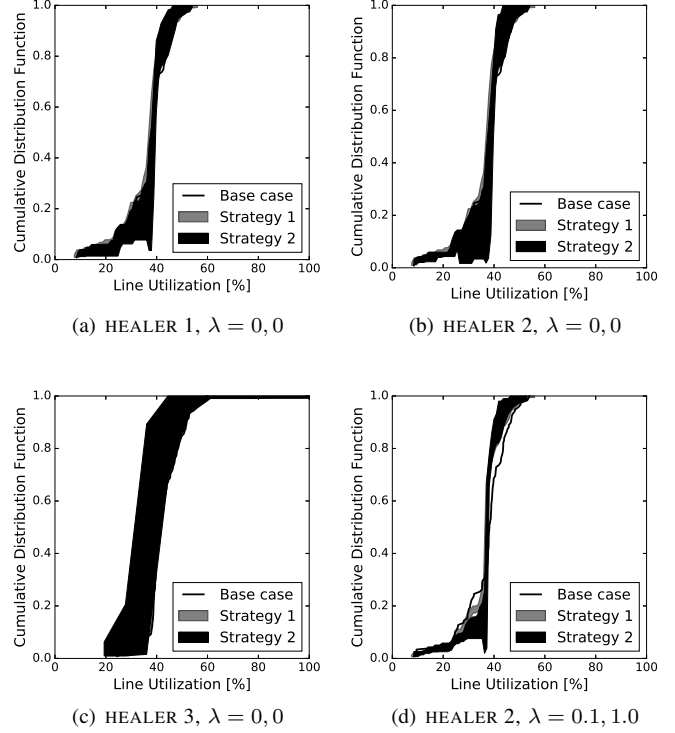
Fig. 6. Lines utilization in case-39 with AC power flow under different healing modes and \lambda values for STRATEGY 1 and STRATEGY 2 respectively.
