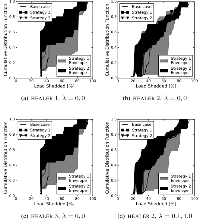
Fig. 3. Load shedded in case-30 with AC power flow under different healing modes and \lambda values for STRATEGY 1 and STRATEGY 2 respectively.
