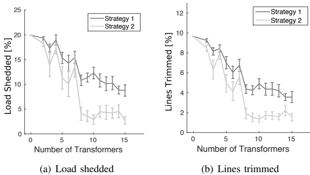
Fig. 8. Load shedded and lines trimmed in case-39 and HEALER 3 with AC power flow and varying number of smart transformers.
