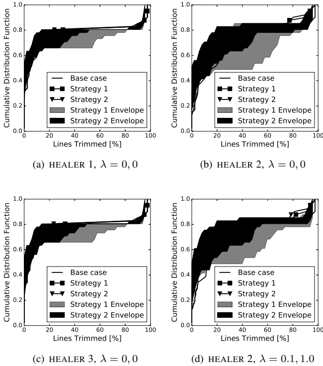
Fig. 5. Lines trimmed in case-30 with AC power flow under different healing modes and \lambda values for STRATEGY 1 and STRATEGY 2 respectively.
