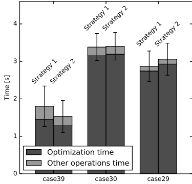
Fig. 9. Computational times for STRATEGY 1 and STRATEGY 2 under HEALER 2 with \lambda = 0 for three power networks.
