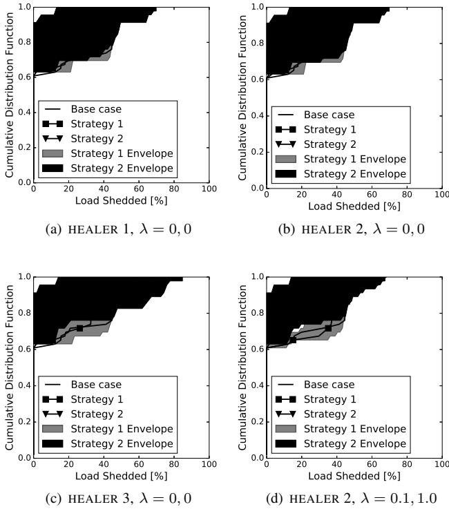
Fig. 2. Load shedded in case-39 with AC power flow under different healing modes and \lambda values for STRATEGY 1 and STRATEGY 2 respectively.
