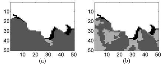
Fig. 7. Classification maps obtained with (a) \tau = 5 and (b) \tau = 5 \times 10^{-5} .
