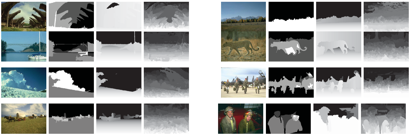
Fig. 13. From left to right. Original image, results of the proposed system, results from [5], and results from [6]. White regions are closer to the viewer, while black ones are further away.
