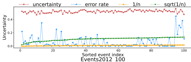
Fig. 1: Statistics of the estimated per-class uncertainty, per-class error rate, the inverse of per-class number 1/n and the sqrt of 1/n on the training sets of Events2012_100.
