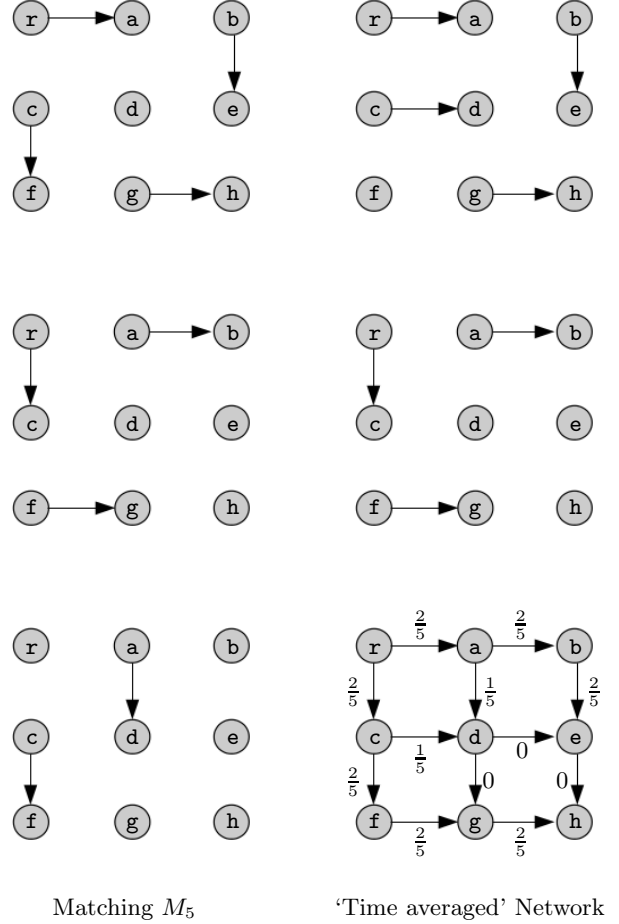
Figure 5: Some feasible activations of the 3 \times 3 grid network which are activated uniformly at random. The components corresponding to each edge in the resulting overall activation vector \beta is denoted by the numbers alongside the edges.
