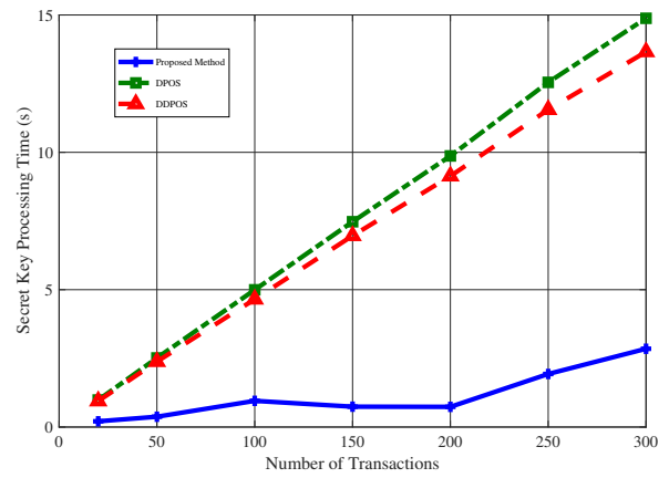
Fig. 9. Key processing time vs the number of transactions.
