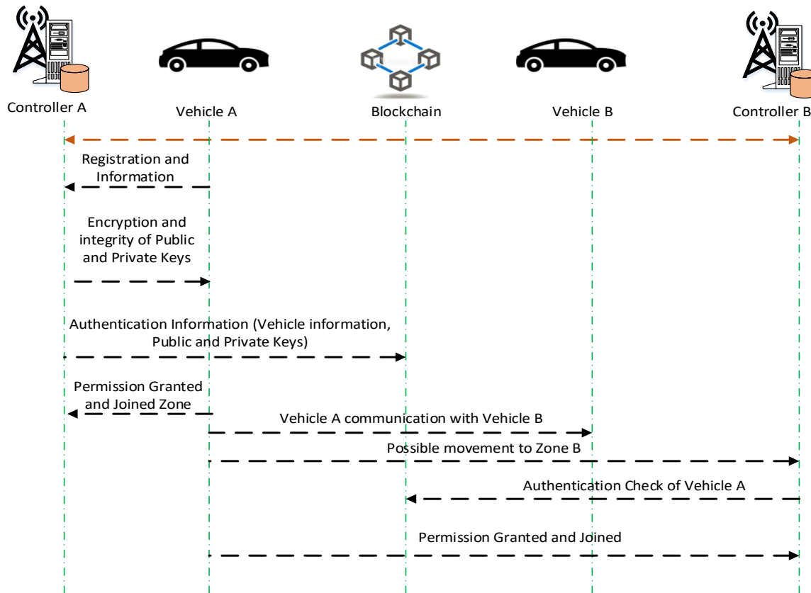
Fig. 5. Registration in a zone in the proposed architecture.
