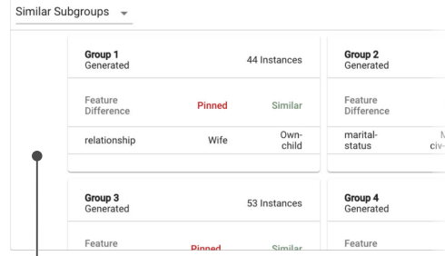
Figure 5: Here we can see the Suggested and Similar Subgroup View for both suggested and similar subgroups. Users can hover over any card to see detailed feature and performance information in the Detailed Comparison View .
