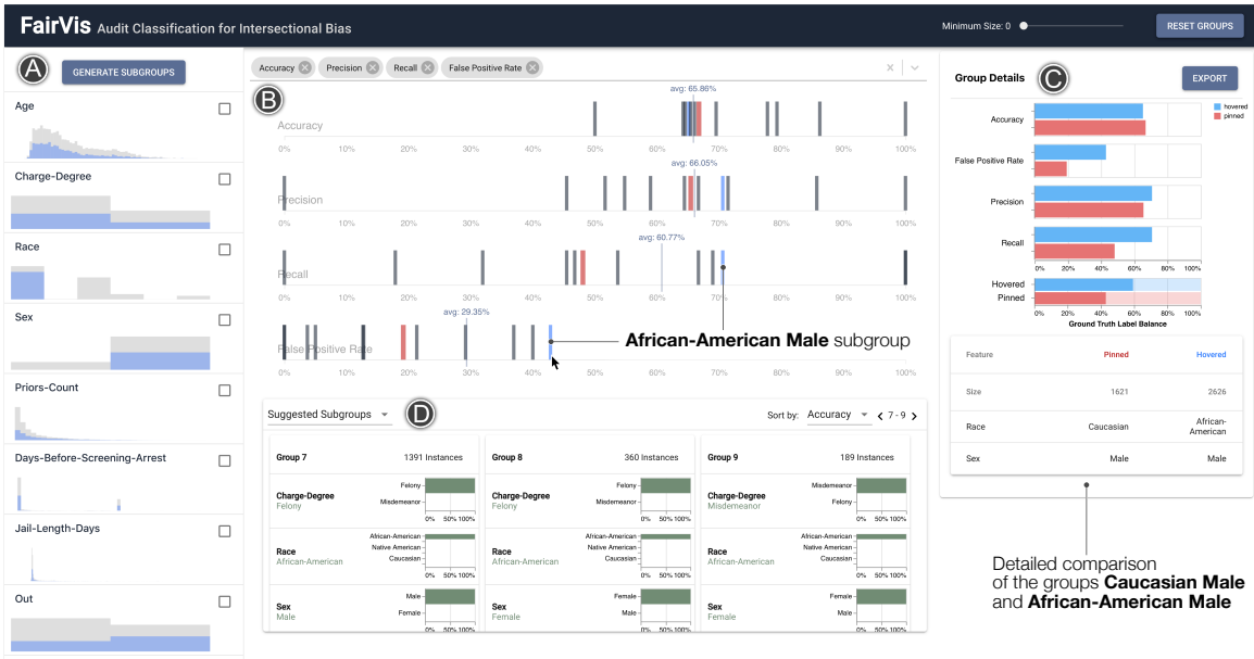
Figure 1: FAIRVIS integrates multiple coordinated views for discovering intersectional bias. Above, our user investigates the intersectional subgroups of sex and race . A. The Feature Distribution View allows users to visualize each feature’s distribution and generate subgroups. B. The Subgroup Overview lets users select various fairness metrics to see the global average per metric and compare subgroups to one another, e.g., pinned Caucasian Males versus hovered African-American Males . The plots for Recall and False Positive Rate show that for African-American Males, the model has relatively high recall but also the highest false positive rate out of all subgroups of sex and race. C. The Detailed Comparison View lets users compare the details of two groups and investigate their class balances. Since the difference in False Positive Rates between Caucasian Males and African-American Males is far larger than their difference in base rates, a user suspects this part of the model merits further inquiry. D. The Suggested and Similar Subgroup View shows suggested subgroups ranked by the worst performance in a given metric.
