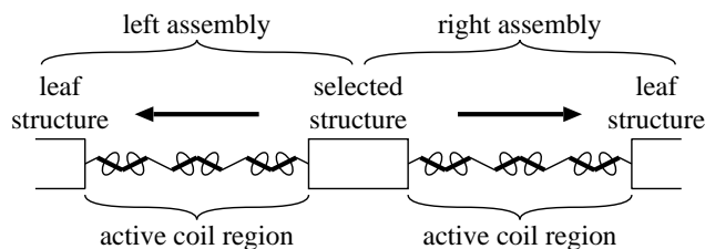
Figure 10: Double linked assembly created by IK algorithm from one active coil region on both sides of the selected structure. Each coil region contains three residues, leading to six rotational joints per coil region. The bold arrows denote assembly direction from root to leaf.
