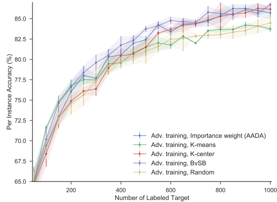
Figure 4: Object classification result (Office D → A). We compare different sampling methods with adversarial training. BvSB and AADA perform the best with 81.3% and 80.7% mean accuracy of 20 rounds separately.
