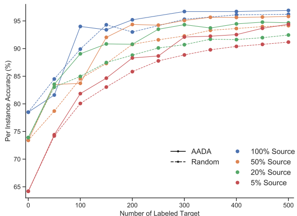
Figure 10: Results on SVHN \rightarrow MNIST with a subset of labeled source data. Using importance weight for sampling is better than random selection, and the improvement is even higher when we have less labeled source data for training.
