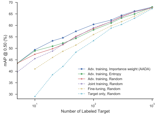
Figure 7: Object detection result (KITTI \rightarrow Cityscapes) after 9 rounds. The x -axis is shown in log scale. The left-most points represent the initial round where no labeled target is available. Our AADA outperforms all other baselines when up to 1000 labeled targets are available.
