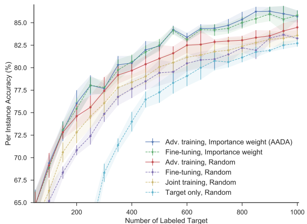
Figure 8: Comparing different training schemes on the Office dataset (D \rightarrow A). Adversarial training with importance weight for sampling (AADA) outperforms other baselines with different training schemes.
