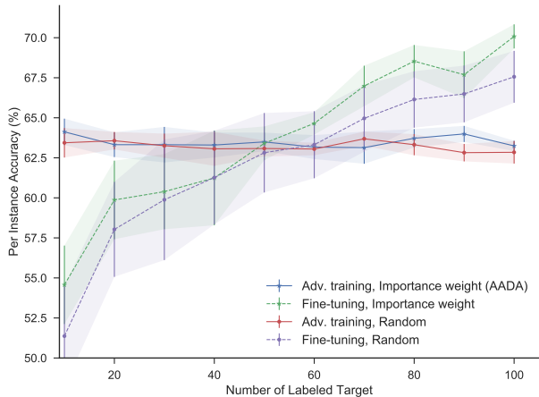
Figure 9: Comparing different training schemes on the VisDA dataset. Using adversarial training, the accuracy does not improve when more labeled targets are added since the target domain in VisDA is closer to ImageNet images for pre-training. However, the accuracy improves when we use fine-tuning, in which using importance weight for sampling is better than random sampling.
