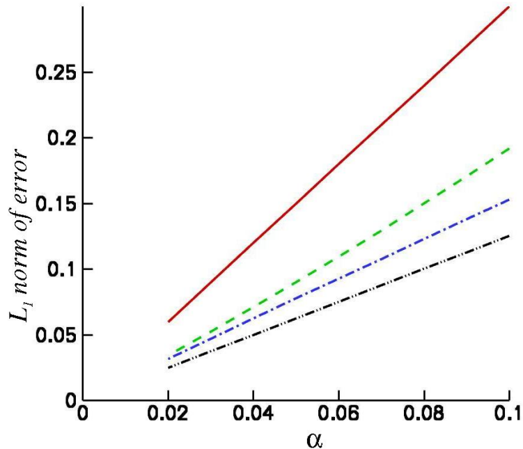
Figure 16: The L_1 norm of the error between the CFB equations' solution and the entropy solution. The error is displayed for four different values of t . t = 0 —, t = 1 ----, t = 2 - · - · - ·, and t = 3 - · - · - · - · - ·. The error approaches zero roughly linearly as \alpha \rightarrow 0 .
