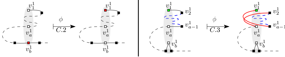
Figure 13: Example of cases C.2 and C.3 of the definition of \phi . Vertices inside the same grey bags correspond to the same vertex of the graph. On the left part of the figure (case C.2), in the initial configuration the vertex v_1^1 is unlabeled and the vertex v_b^1 is labeled (with color red) and the application of \phi in this case exchanges this label from v_b^1 to v_1^1 . On the right part of the figure, v_b^1 is a digon and therefore it is unlabeled and by cases C.1 and C.2, v_1^1 has to be labeled (depicted in green).
