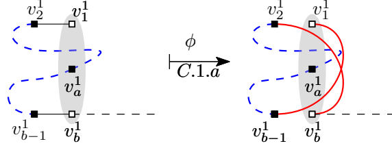
Figure 10: Example of case C.1.a of the definition of \phi . All vertices inside the grey bag are different occurrences of the same vertex v_1^1 of the graph. The vertices v_1^1 and v_b^1 are unlabeled and the black vertices v_2^1 , v_a^1 , and v_{b-1}^1 can be either labeled or unlabeled.
