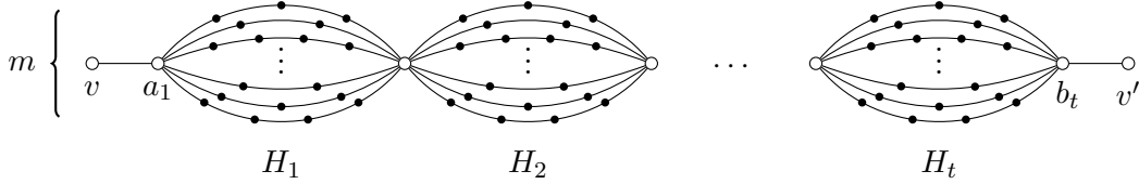
Figure 4: Construction of the graph G .
