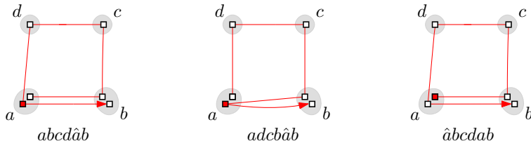
Figure 1: An illustration of the walks abcd\hat{a}b , \overleftarrow{abcd\hat{a}b} = adcb\hat{a}b , and \hat{a}bcdab . The grey bags correspond to vertices of the graph. The squares are copies of the corresponding bag-vertex and these together with the red path illustrate the order the vertices appear in the walk. Red squares correspond to labeled vertices.
