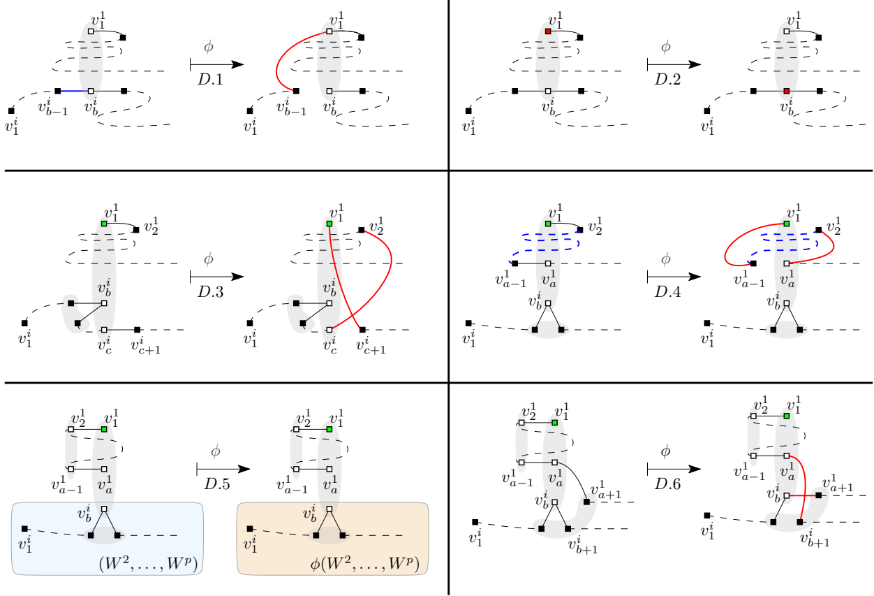
Figure 16: Example of cases D.1-D.6 of the definition of \phi . In each grey bag, all vertices inside the corresponding bag are the same vertex of the graph. Labeled vertices are depicted in red and green. White vertices correspond to unlabeled vertices and black vertices can be either labeled or unlabeled.
