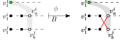
Figure 9: Example of case B of the definition of \phi . All vertices inside the grey bag are different occurrences of the same vertex v_1^1 of the graph. The white vertices v_a^i and v_b^j are unlabeled, the black vertices could be labeled or unlabeled, and the green vertex v_1^1 is labeled in this specific example.
