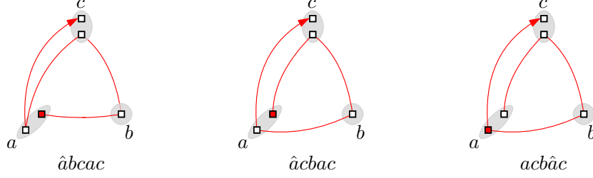
Figure 2: An illustration of the walks \hat{a}bcac , \hat{a}\overleftarrow{b}cac = \hat{a}cbac , and acb\hat{a}c . The grey bags correspond to vertices of the graph. The squares are copies of the corresponding bag-vertex and these together with the red path illustrate the order the vertices appear in the walk. Red squares correspond to labeled vertices.
