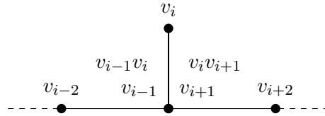
Figure 5: An example of a labeled walk W with a digon i .
