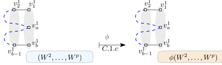
Figure 12: Example of case C.1.c of the definition of \phi . All vertices inside the grey bags correspond to the same vertex of the graph. By case C.1.a, the blue subwalk W^1[2, b - 1] is palindrome, and therefore by Lemma 7 , the vertices in it are unlabeled.
