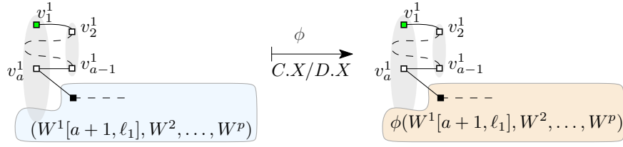
Figure 15: Examples of cases C.X and D.X of the definition of \phi .
