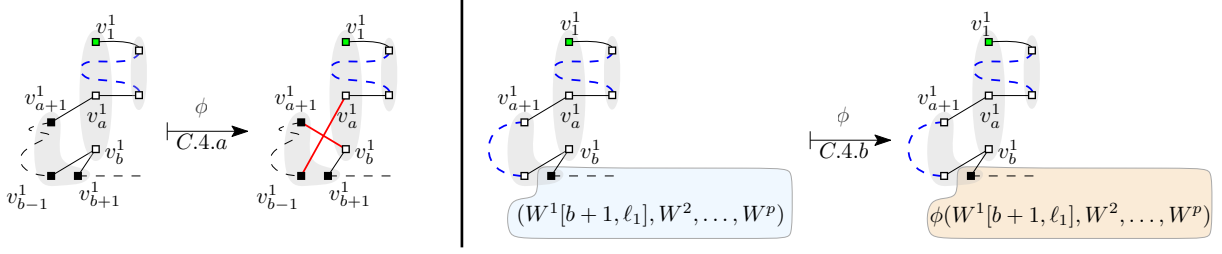
Figure 14: Examples of cases C.4.a and C.4.b of the definition of \phi . By case C.2, b is a digon on W^1 and by case C.3, W^1[2, a-1] is a palindrome. For both case C.4.a and case C.4.b, we have that v_{a+1}^1 = v_{b-1}^1 ( v_{a+1}^1, v_{b-1}^1 , and v_{b+1}^1 are in the same grey bag). If W^1[a+1, b-1] is not a palindrome, then we are in case C.4.a (on the left), while if W^1[a+1, b-1] is a palindrome, we are in case C.4.b. (on the right).
