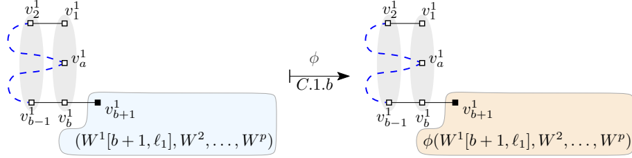
Figure 11: Example of case C.1.b of the definition of \phi . All vertices inside the grey bags are the same vertex of the graph. By case C.1.a, the blue subwalk W^1[2, b-1] is palindrome, and therefore by Lemma 7 , the vertices in it are unlabeled.
