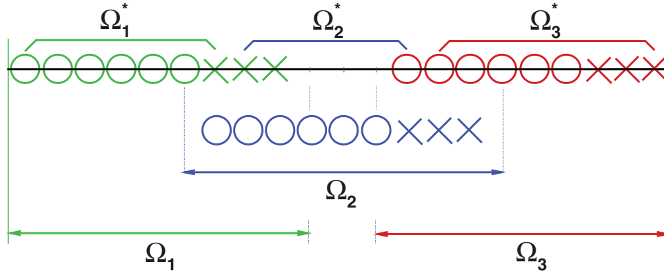
FIG. 2.2. RAS ( n_{domain} = 3 , n_{overlap} = 4 - 1 , n_{xpt} = 6 ; see section 4.1 for these parameters). The circles and crosses stand for the unknowns in each subdomain.
