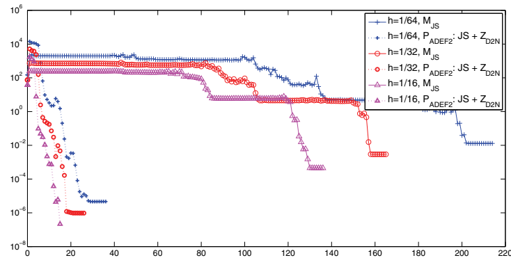
FIG. 4.5. Case HPL3 with various mesh sizes: 1/64 (crosses), 1/32 (circles), and 1/16 (triangles); n_{overlap} = 1 , n_{domain} = 16 . Z_{D2N} : dotted lines, JS: solid lines.
