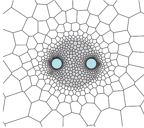
FIG. 4. Coarsened version of one of the unstructured meshes based on Voronoi dual control volumes employed in the numerical computation of the exact time periodic thermal response of single U-pipe borehole configurations by means of a first order finite volume discretization of the governing equations.
