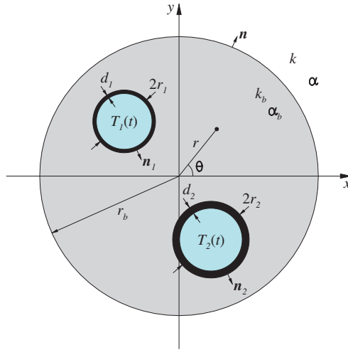
FIG. 1. Cross section of a typical geothermal borehole of radius r_b with a single U-shaped pipe in it and filled with a grout material with thermal conductivity k_b and thermal diffusivity \alpha_b that in general differ from the corresponding values k and \alpha of the surrounding ground.
