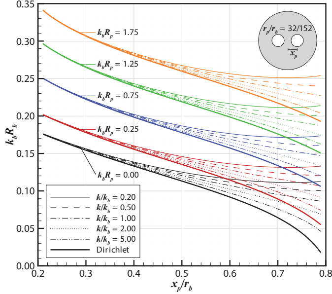
FIG. 2. Nondimensional borehole thermal resistance k_b R_b for a thermally symmetric single U-pipe borehole configuration with pipe and borehole diameters equal to 32 mm and 152 mm, respectively, as a function of the nondimensional distance x_p/r_b of the pipe centers to the borehole center, the nondimensional ratio of thermal conductivities k/k_b , and the nondimensional inner thermal resistance k_b R_p of the pipes. Also represented, with thicker lines, are the values obtained through the imposition of the Dirichlet boundary condition at the borehole wall instead of the asymptotic matching condition at infinity.
