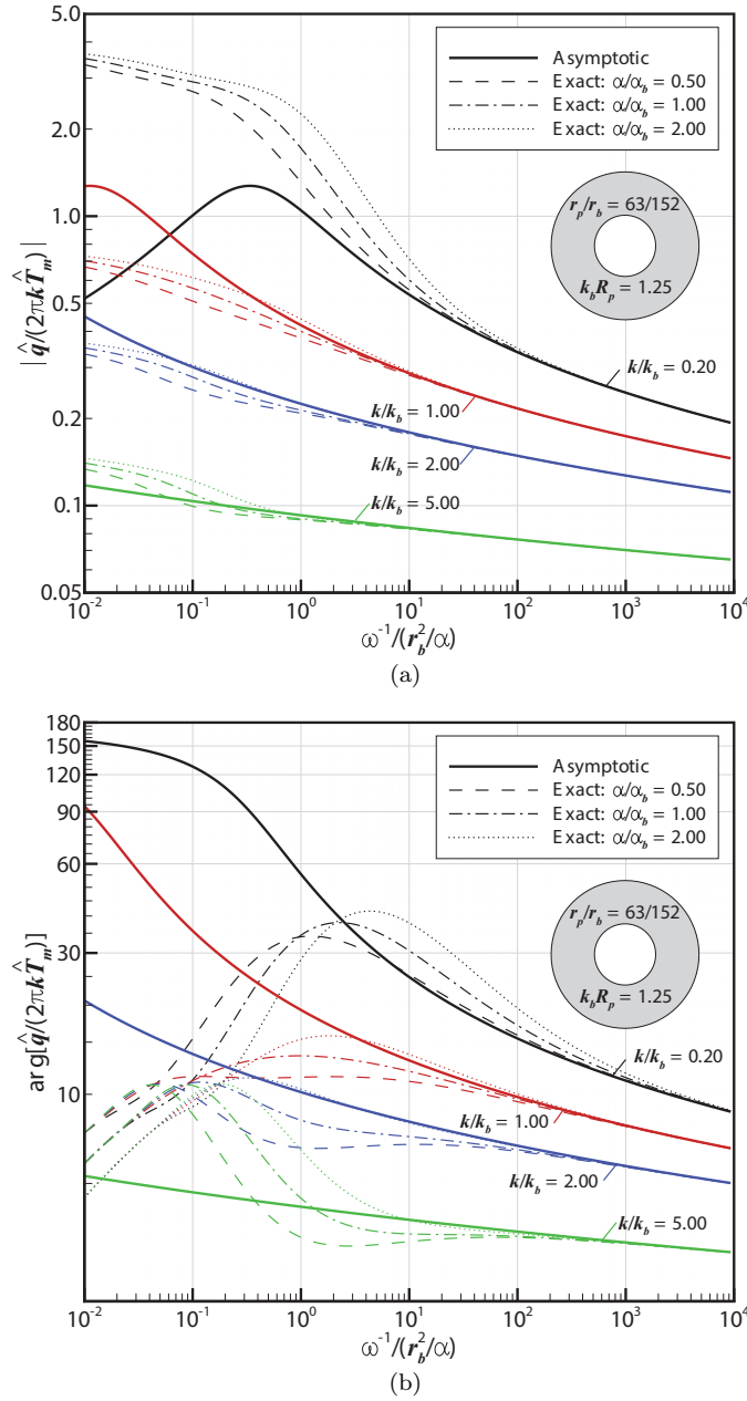
FIG. 3. (a) Modulus and (b) argument (in degrees) of the nondimensional heat injection rate per unit borehole length \hat{q}/(2\pi k \hat{T}_m) for a pipe-in-pipe coaxial borehole configuration with pipe and borehole diameters equal to 63 mm and 152 mm, respectively, and a nondimensional inner thermal resistance of the pipes of k_p R_p = 1.25 as functions of the ratio between the characteristic time of variation \omega^{-1} of the mean fluid temperature T_m and the characteristic transverse diffusion time r_b^2/\alpha of the borehole and for different values of the ratio of thermal conductivities k/k_b . Shown are the values corresponding to the asymptotic solution (continuous lines) and the exact analytical solutions for different values of the ratio of thermal diffusivities \alpha/\alpha_b (discontinuous lines).
