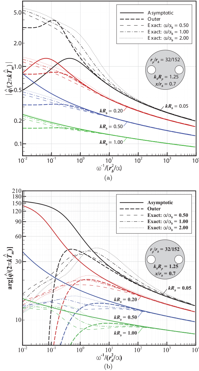
FIG. 5. (a) Modulus and (b) argument (in degrees) of the nondimensional heat injection rate per unit borehole length \hat{q}/(2\pi kT_m) for a thermally symmetric single U-pipe borehole configuration with pipe and borehole diameters equal to 32 mm and 152 mm, respectively, nondimensional pipe center distance to borehole center of x/r_b = 0.70 , and a nondimensional inner thermal resistance of the pipes of k_p R_p = 1.25 as functions of the ratio between the characteristic time of variation \omega^{-1} of the mean fluid temperature T_m and the characteristic transverse diffusion time r_b^2/\alpha of the borehole and for different values of the nondimensional borehole thermal resistance kR_b . Shown are the values corresponding to the asymptotic expression (thick continuous lines), the expression obtained from imposing the outer solution at r = r_b (thick dashed lines), and the numerically obtained exact solution for different values of the ratio of thermal diffusivities \alpha/\alpha_b (other discontinuous lines).
