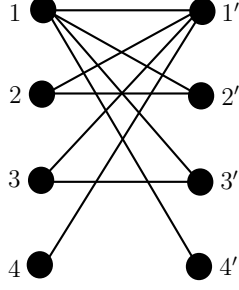
Figure 3: A graph H where for any choice of the parameters \alpha, \beta , the set of dominating bicliques \mathcal{C}_{\alpha, \beta} consists either of a single extremal biclique or of the two extremal and two non-extremal bicliques. Namely, when \alpha > \beta (resp. \alpha < \beta ) we have that the unique element of \mathcal{C}_{\alpha, \beta} is the extremal biclique (\{1, 2, 3, 4\}, \{1'\}) (resp. (\{1\}, \{1', 2', 3', 4'\}) ); when \alpha = \beta we have that \mathcal{C}_{\alpha, \beta} consists of the bicliques (\{1\}, \{1', 2', 3', 4'\}) , (\{1, 2, 3, 4\}, \{1'\}) , (\{1, 2\}, \{1', 2'\}) and (\{1, 3\}, \{1', 3'\}) .
