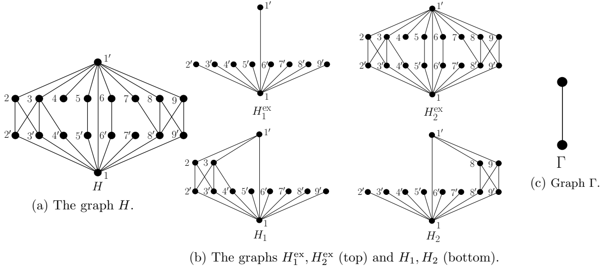
Figure 7: An example of a graph H which falls into Case 3 of our analysis.
