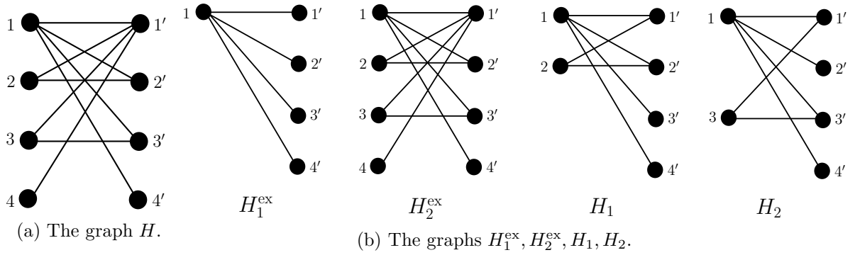
Figure 6: An example of a graph H which falls into Case 2 of our analysis.
