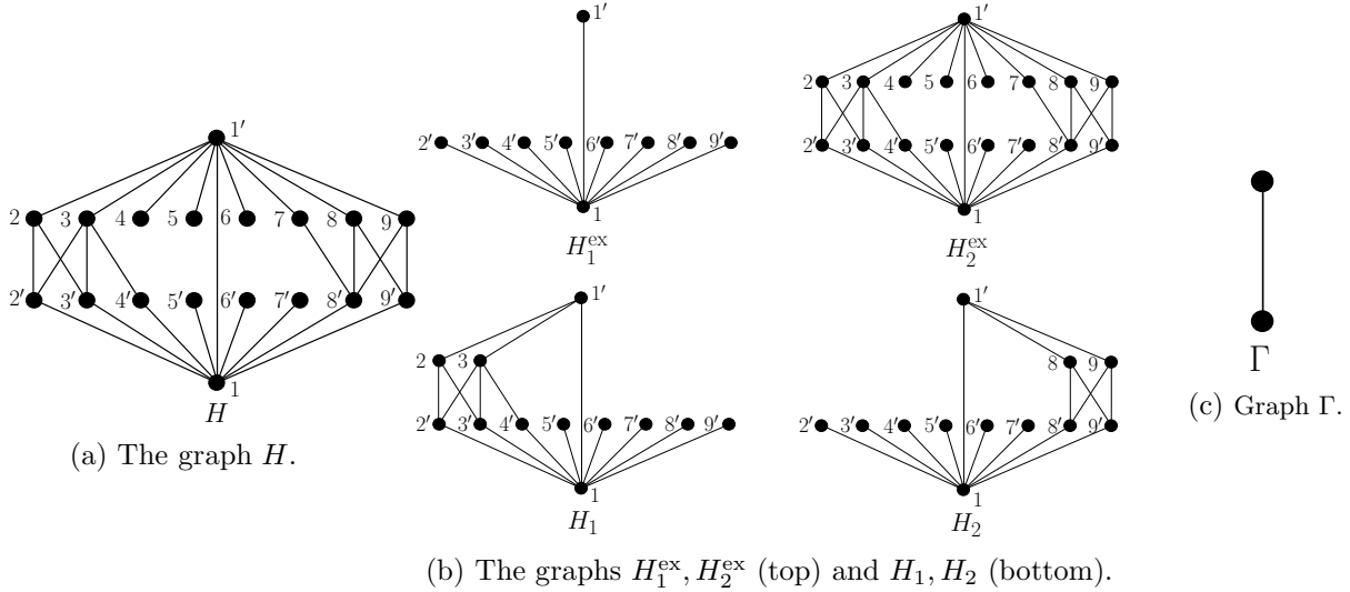
Figure 5: An example of a graph H which falls into Case 1 of our analysis.
