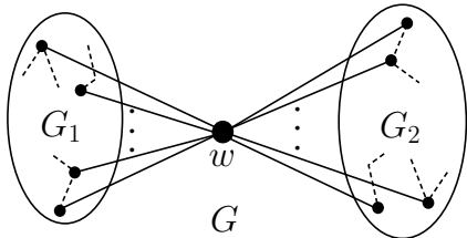
Figure 2: “Gluing” the reductions ([7])
