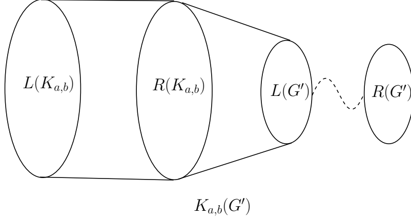
Figure 4: The reduction for Item 2
