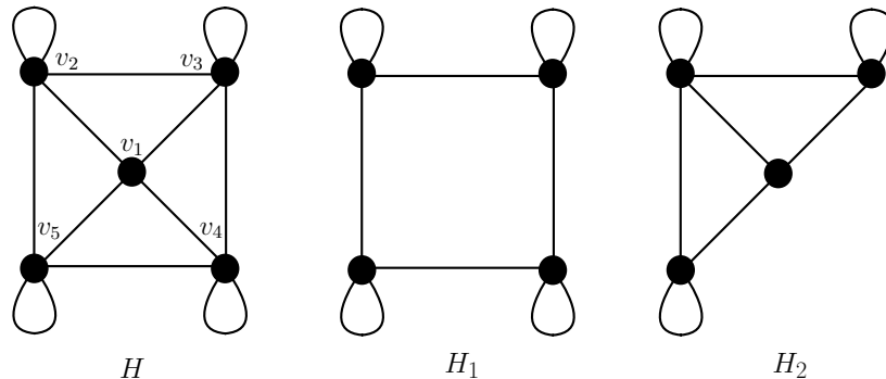
Figure 1: Example of a graph H and the subgraphs induced by the neighbourhoods of its (maximum degree) vertices.
