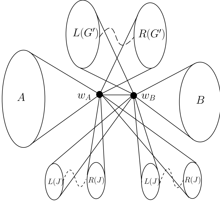
Figure 8: The graph G
