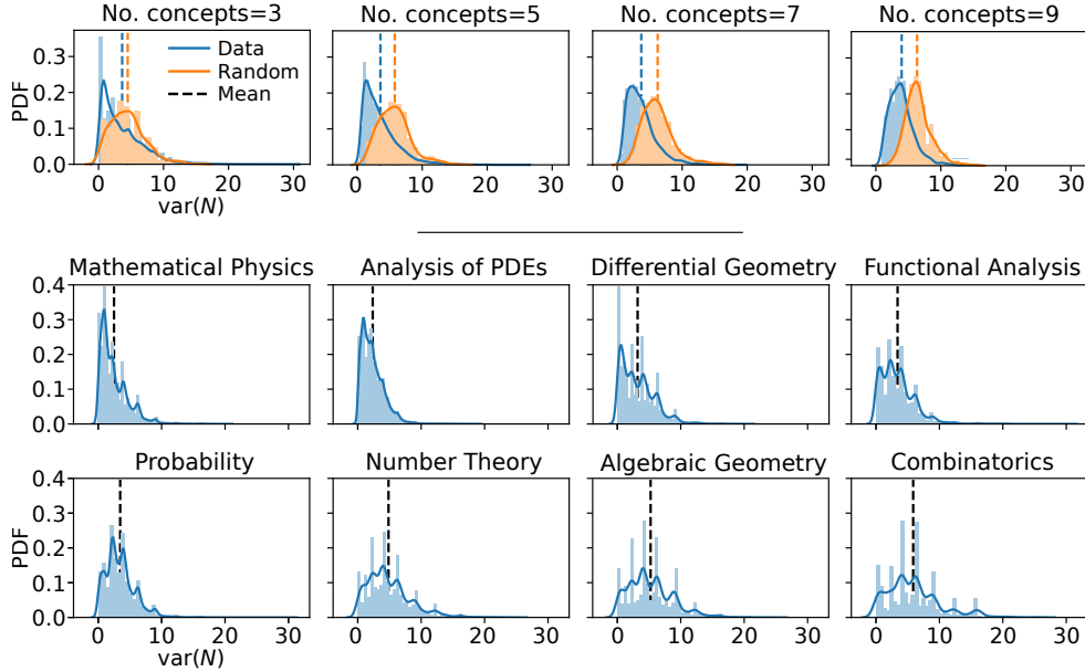
FIG. 3. (Top figure) Distribution of network variances of concept distributions p^{(i)} in papers, calculated with respect to the geodesic distance in the Wikipedia network. In each panel, the probability density function (pdf) of variances is calculated for papers containing 3 (resp. 5, 7, 9) concepts present in the Wikipedia network, and is compared with the variance pdf for a collection of (null model) virtual papers with the same number of concepts. The empirical variance distributions are concentrated on smaller variances compared to the null model variances, as confirmed by the one-sided Mann-Whitney U test (see Appendix C). (Bottom figure) Distribution of network variances of concept distributions p^{(i)} for arXiv papers from different sub-fields. The fields are ordered from top left to bottom right according to concentration on increasing variances as found from the Mann-Whitney U test.
