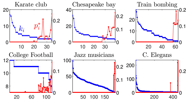
FIG. 8. Degree sequence (blue) and maximum variance distribution (red) on a number of real-world networks from the KONECT database [28]. The horizontal axis contains node indices i , sorted according to decreasing degree. For each node, the degree k_i and maximum variance probability p_i^* are given, with scales on the left and right vertical axis, respectively.
