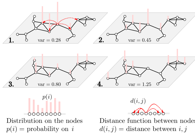
FIG. 1. The variance of distributions on a graph can be defined with respect to a distance function between the nodes of the graph. This measure allows us to compare how ‘spread out’ different distributions are on the network. In the example above, the distributions become more spread out over the network, going from distribution 1. \rightarrow 4. with an increasing variance as a result; here, the variance is calculated with respect to the square root resistance distance as in equation (2.3).
