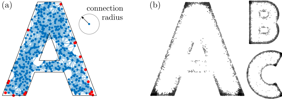
FIG. 5. The maximum variance support of random geometric graphs (RGGs) in a bounded domain is more likely to contain nodes which are located near the boundaries. Panel (a) shows one realization of an RGG on n = 500 nodes in a domain shaped as the letter ‘A’, with connection radius as indicated. The nodes in the maximum variance support are colored red, and are all located near the boundary of the domain. Panel (b) summarizes the maximum variance support node locations calculated in 250 independent RGG realizations on the given domains. A darker (resp. lighter) shading indicates a higher (lower) density of maximum variance nodes. This figure seems to confirm that the maximum variance support nodes are more likely to be located near the domain boundaries and, in particular, near corners with ‘high curvature’.
