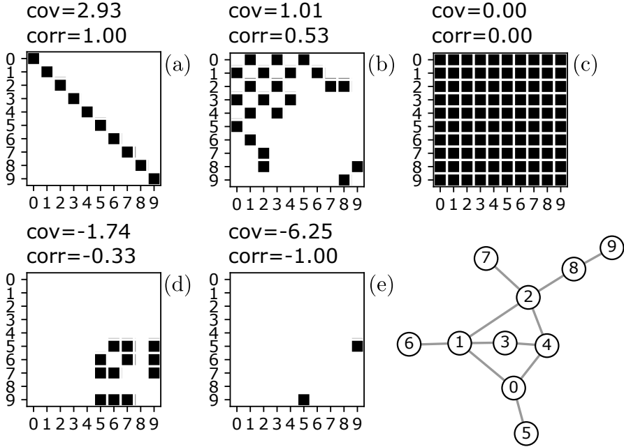
FIG. 7. Five joint distributions on a small, 10-node graph. Each joint distribution is illustrated by a 10 \times 10 grid with white squares indicating P(i, j) = 0 and black squares a constant P(i, j) = p such that P normalizes. The covariance and correlation are calculated with respect to the shortest path distance for (a) the joint distribution for two identical nodes (N, N) with uniform distribution, (b) joint distribution for the random ends of a link, i.e. (N, M) is a link sampled uniformly at random from the graph, (c) the uniform joint distribution, corresponding to two independent uniform random nodes (d) joint distribution for a pair of leaf nodes, i.e. with (N, M) a random (distinct) pair of nodes from \{5, 6, 7, 9\} and (e) joint distribution for a randomly permuted pair of nodes (N, M) = (5, 9) or (9, 5) .
