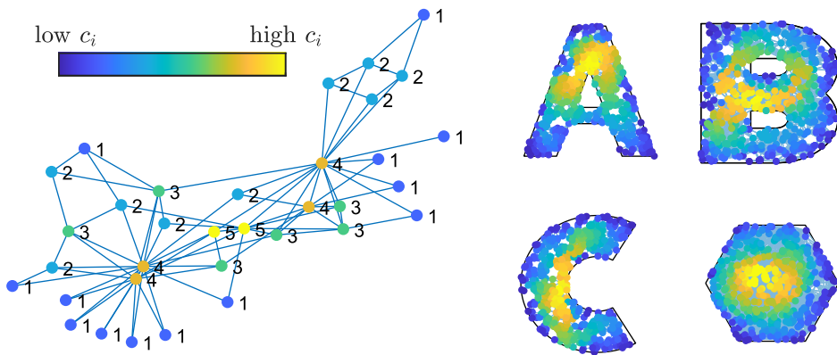
FIG. 6. The iterated core-periphery decomposition divides the nodes of a graph into layers of increasing centrality or ‘coreness’. The figure above shows the coreness c_i of nodes in the Karate club network (obtained from the KONECT database [28]) and four random geometric graphs (see Section 5.1).
