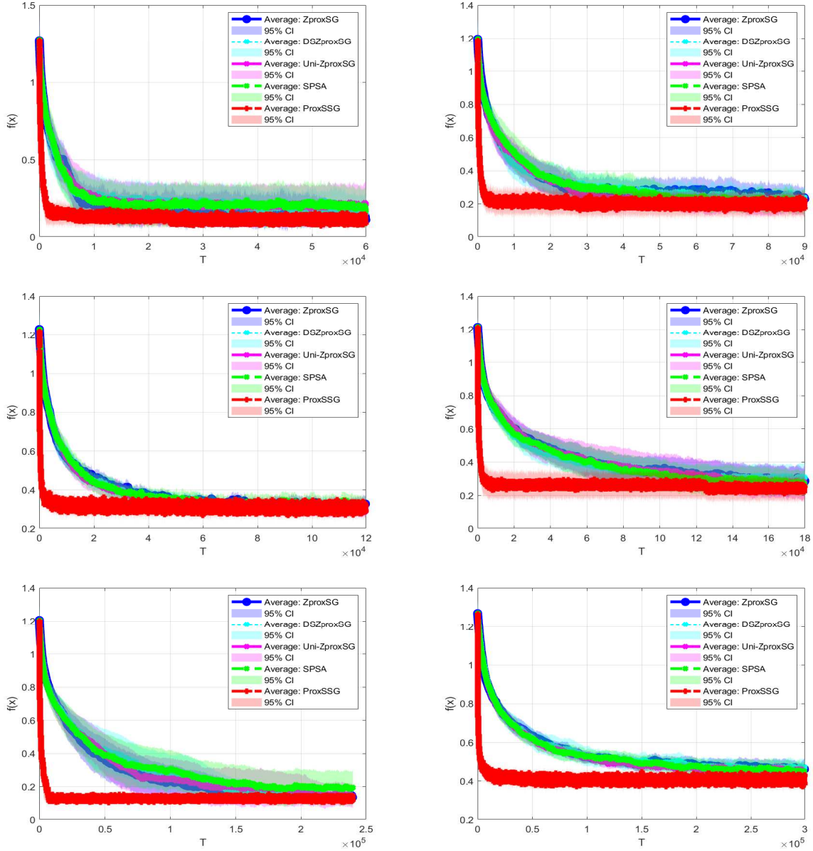
Figure 1: Convergence profiles for Z-ProxSG, DSZ-ProxSG, Uni-ZproxSG, SPSA and ProxSSG: average objective function value (lines) and 95% confidence intervals (shaded regions) vs number of iterations. The upper row corresponds, from left to right, to (d, m) = (10, 30), (20, 45) . The middle row corresponds, from left to right, to (d, m) = (40, 60), (35, 90) . The lower row corresponds, from left to right, to (d, m) = (30, 120), (80, 150) .
