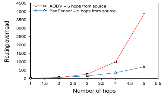
Figure 4: Comparison of AODV and BeeSensor routing overheads at different hops from the source node.
