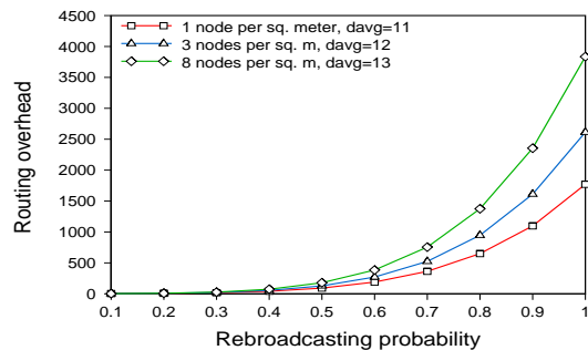
Figure 3: Routing overhead for varying rebroadcasting probabilities ( p_r ).
