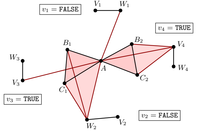
Figure 11: Satisfying assignment for formula E = (v_1 v \neg v_2 v \neg v_3) \wedge (v_1 v v_2 v v_4) and corresponding homological simplification of (K, L) .
