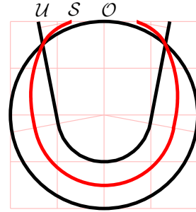
Figure 2: The angle between the two bars in shape \mathcal{U} is adjusted such that d_H(S, \mathcal{O}) = d_H(S, \mathcal{U}) = \frac{1+\eta}{2} .
