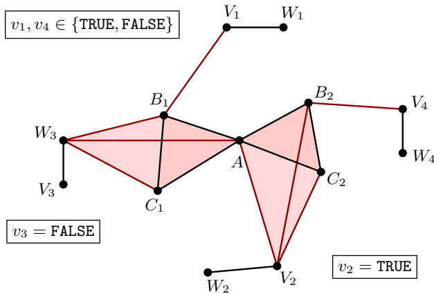
Figure 10: A homological simplification of the pair (K, L) drawn in Figure 9 and output by the reduction of formula E = (v_1 v \neg v_2 v \neg v_3) \wedge (v_1 v v_2 v v_4) . Corresponding satisfying assignments for E .
